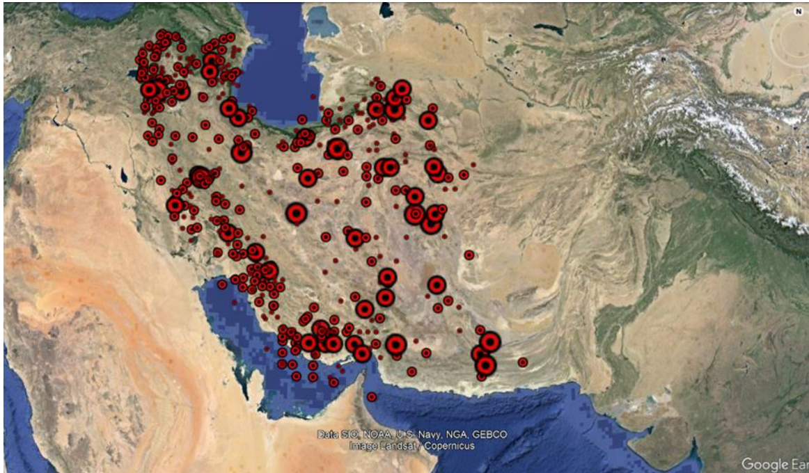
Figure 1: Recorded earthquakes 1900-1963
